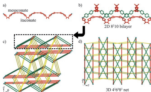
Figure 2. a) 1D arch-bridge-like chain in 1Y . b) 2D bilayer in 1Y . c, d) Schematic representations of the 3D 4^2 6^6 8^2 net. Rods in (c) and (d): green: 4,4'-bipy ligands with N31 atoms; red: carboxylate ligands; yellow: 4,4'-bipy ligands with N41 atoms.
